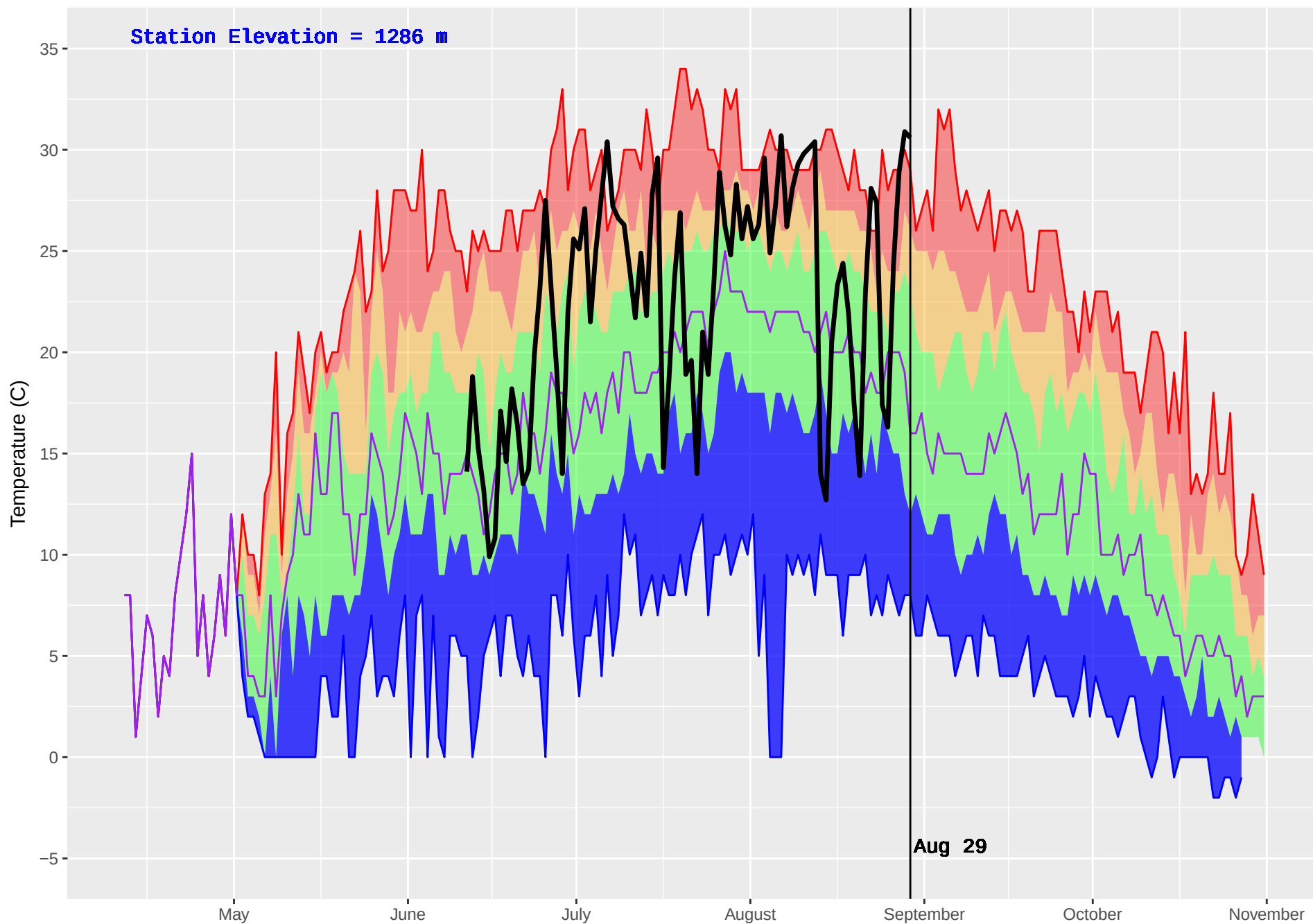
CURWEN CREEK (352) : Historical (1979–2016) and Current (2017) Noon Temperature
