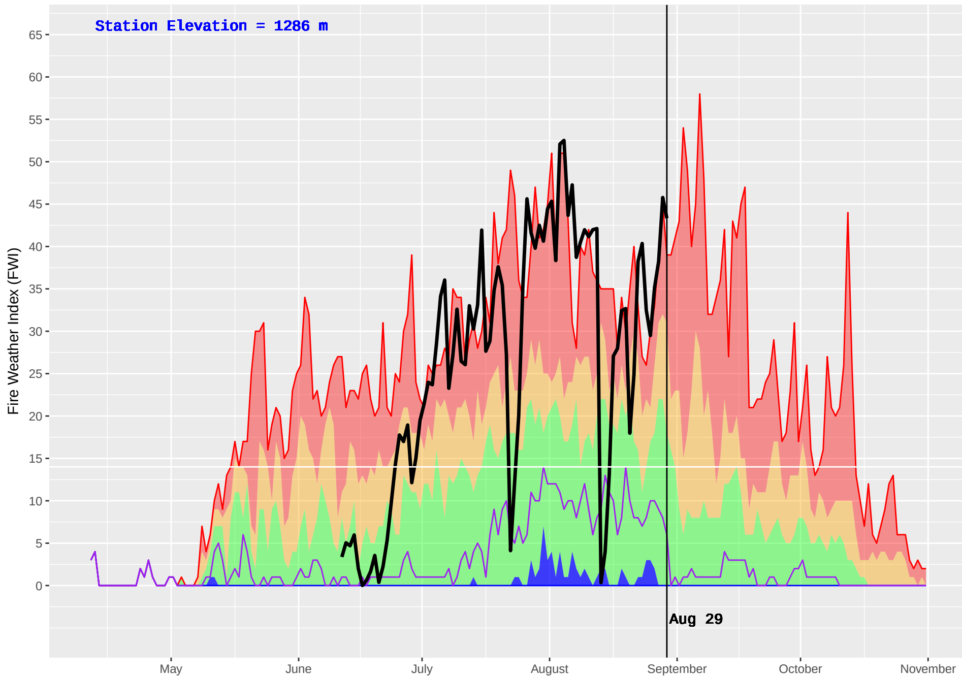
CURWEN CREEK (352) : Historical (1979–2016) and Current (2017) Noon Fire Weather Index (FWI)
