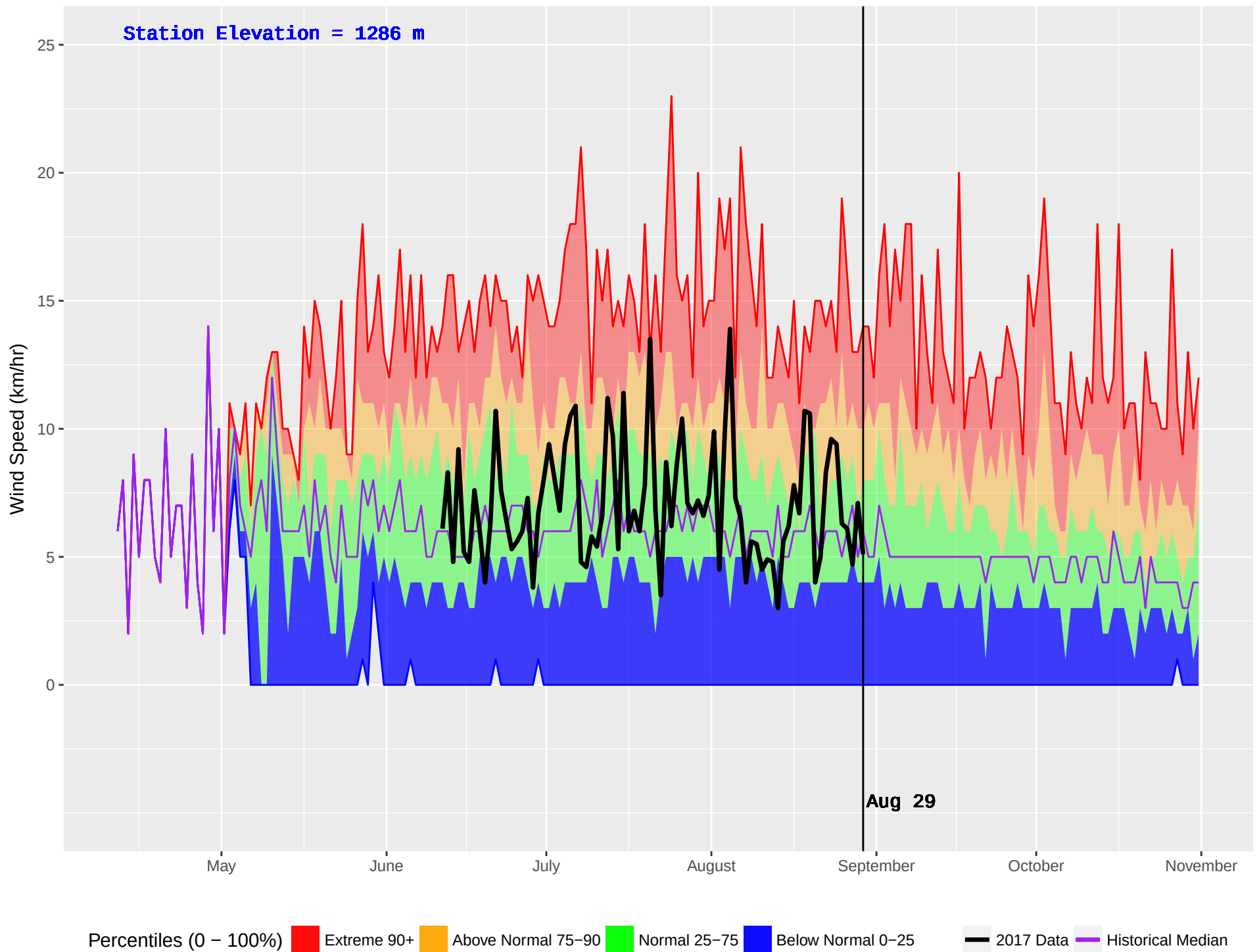
CURWEN CREEK (352) : Historical (1979–2016) and Current (2017) Noon Wind Speed
